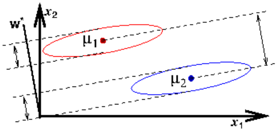
Figure 7.5: Fisher's LDA.
