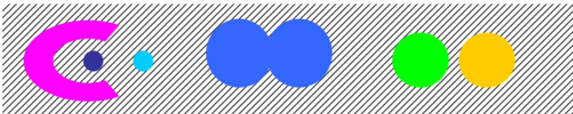
Figure 8.8: 6 density-based clusters.
