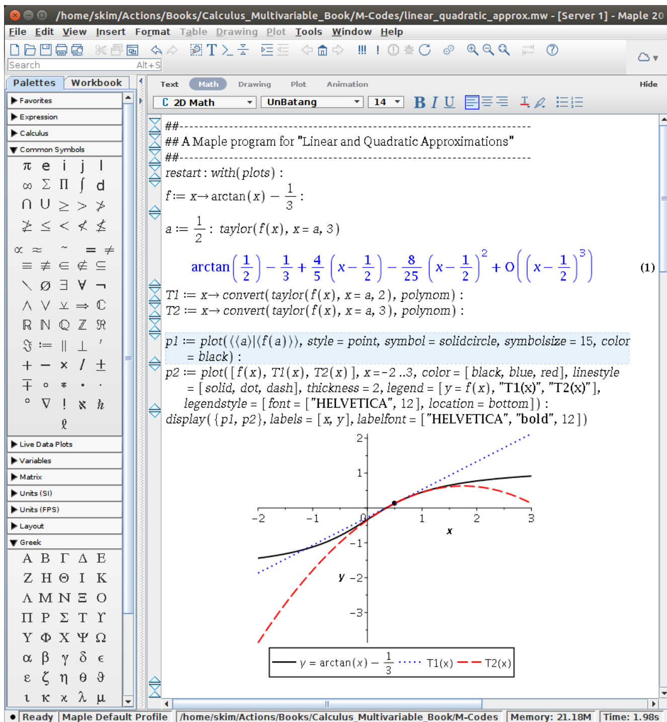
Figure 14.18: Screen-shot of Maple window, which plots linear and quadratic approximations of f(x) = \arctan(x) - \frac{1}{3} about a = \frac{1}{2} .
