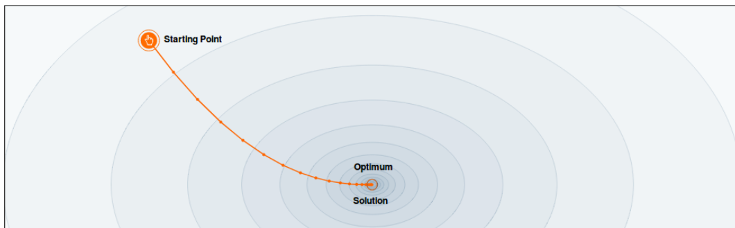
Figure 17.10: On a well-conditioned quadratic function, the gradient descent converges in a few iterations to the optimum. Adding the backtracking line search strategy for the step length does not change much in this case.
