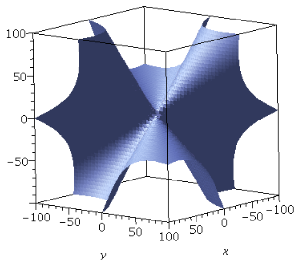
Figure 14.8: implicitplot3d in Maple: a plot of surface defined in Problem 14.33.
